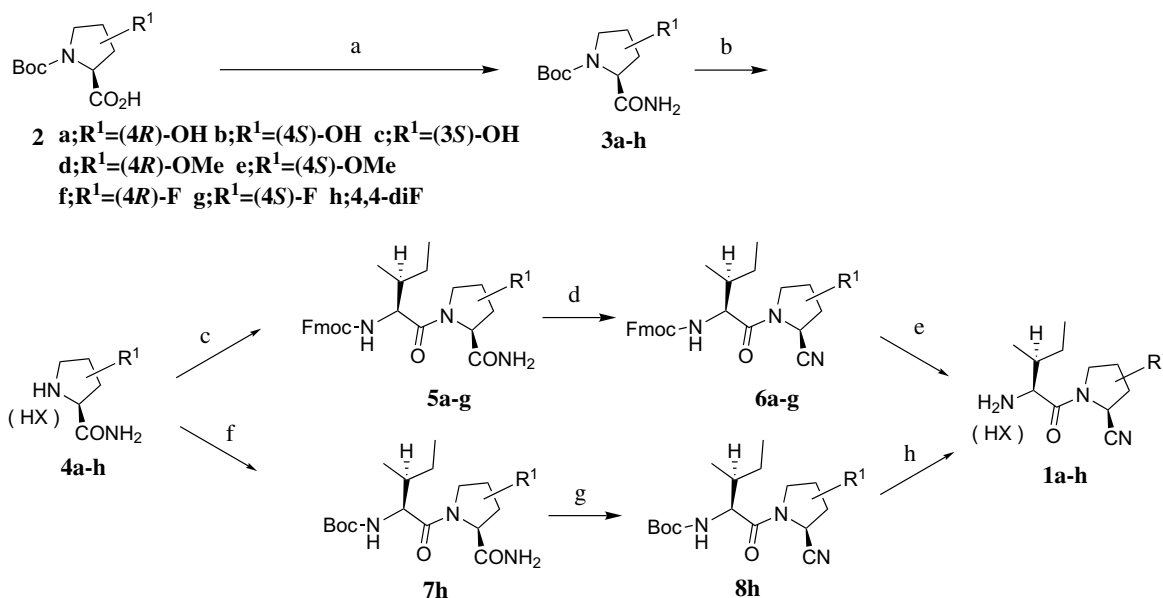
Scheme 1. Reagents: (a) EDC, HOBT, NH 3 , DMF or CH 3 CN; (b) 4M HCl/AcOEt or 4M HCl/1,4-dioxane; (c) Fmoc-L-isoleucine, EDC, HOBT, N,N -diisopropylethylamine, DMF or CH 3 CN; (d) (CF 3 CO) 2 O, THF; (e) Et 2 NH, 1,2-dichloroethane; then HCl; (f) Boc-L-isoleucine, EDC, HOBT, N,N -diisopropylethylamine, THF–DMF; (g) cyanuric chloride, DMF; (h) 2M HCl.
